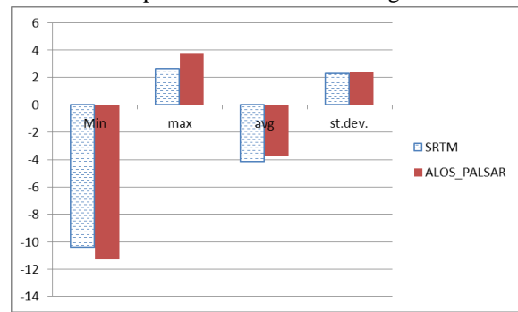
Fig 2. ( H_{\text{field}} - H_{\text{SRTM1, ALOS/PALSAR}} )
