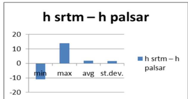
Fig 18. Test area 2, (h SRTM1 - h ALOS/PALSAR), units in meters.
